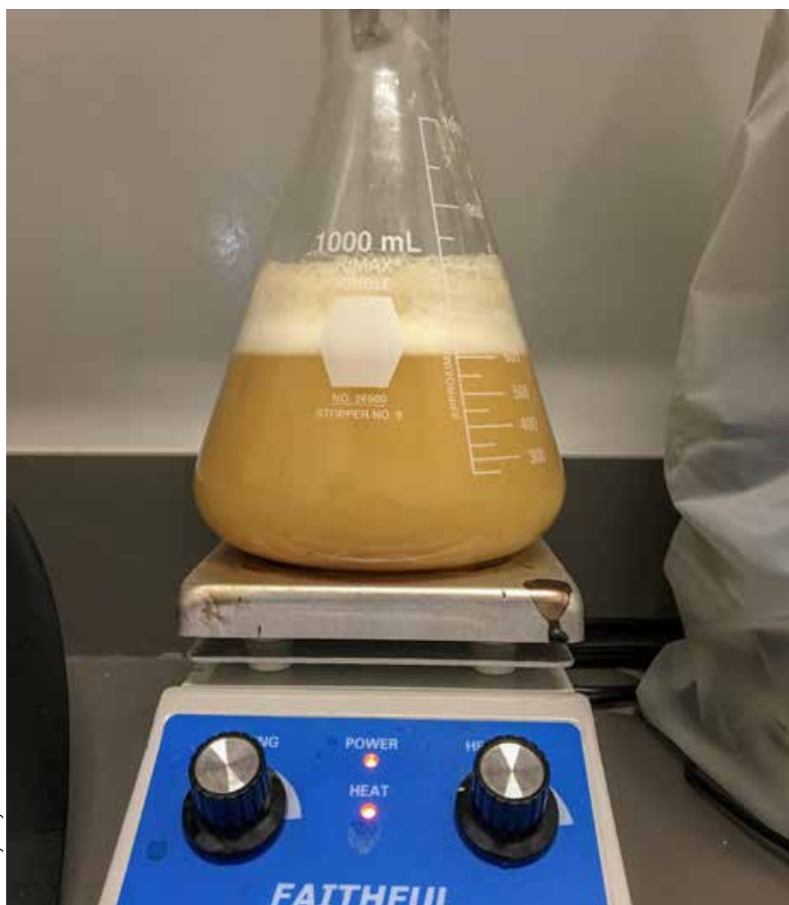
A forced ferment test will show the potential final gravity of a full fermentation within 2–3 days using a heated stir plate.
